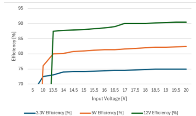
Fig. 3. The efficiency graph of the LM2596 regulator while ramping up the input voltage stopping at 20 volts.
