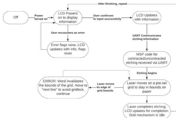
Fig. 6. MSP430FR2355 State Diagram demonstrating the operations the MSP will be performing
