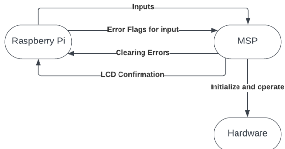
Fig. 5. Interpretation of how data flows through the two microcontrollers and to the system for instruction.
