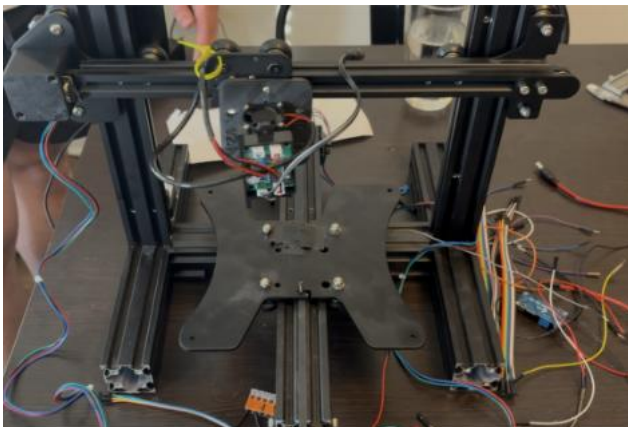
Fig. 1. Picture of the assembled gantry system
